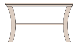
NODA Cocktail Table (Curved Legs) ITEM# NOD-32-02 34"W x 20"D x 20"H
