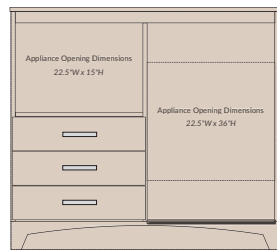
NODA Micro-Fridge Unit - NO Trim ITEM# NOD-32-14 48"W x 22"D x 43"H
